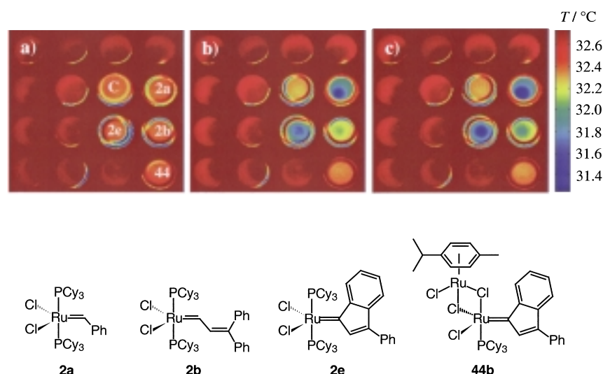
Figure 2. Parallel screening of four different ruthenium catalysts with IR-thermography as the detection method. [64] The test reaction is the cyclization of 1,7-octadiene to cyclohexene. The tube marked “C” shows a control experiment in which catalyst 2a is added to octane instead of the octadiene. a) Before addition of the catalysts; b) after 1 min of reaction time; c) after 2 min of reaction time.
